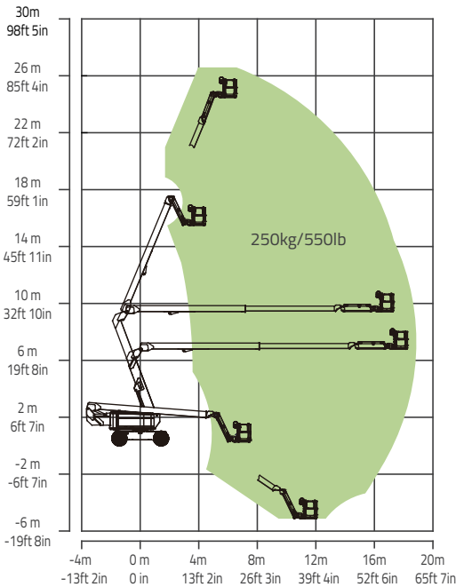
Range of Motion ZA80J
